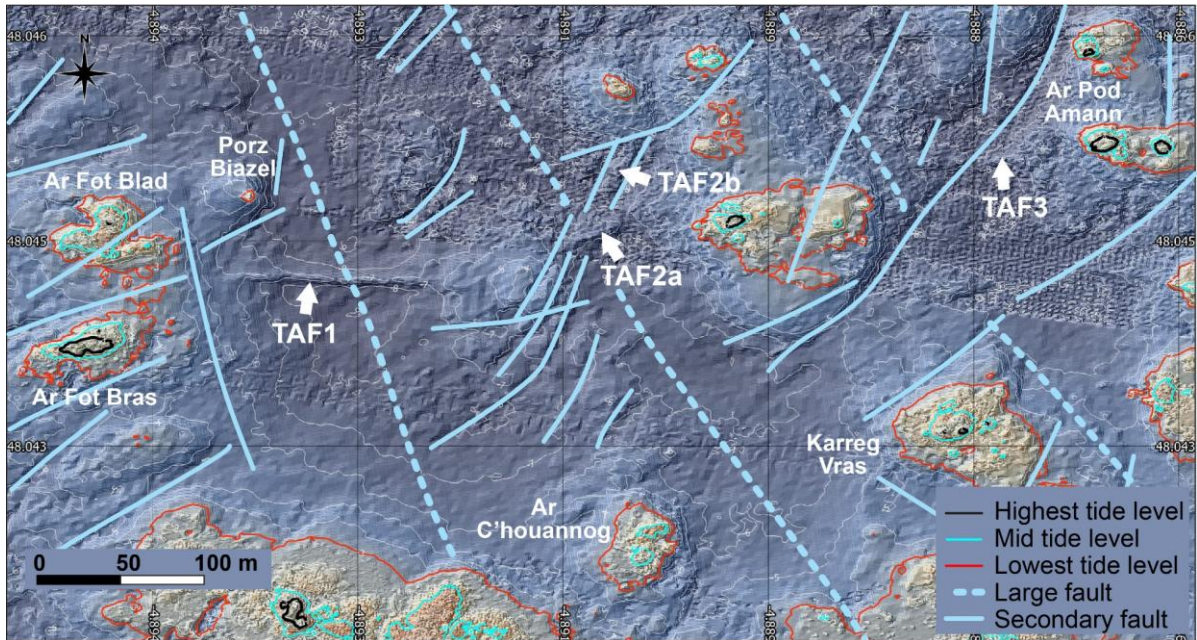
Figure 5. Faults present in the Toul ar Fot sector. Light blue dotted lines represent large NW-SE regional faults over the entire granitic plateau (see Figure 1 for location). These faults form more or less straight depressions that create the channels between the north and south of the granitic ridge. Solid blue lines correspond to secondary NE-SW faults. The directions of TAF1, TAF2A, and TAF3 are oblique in relation to these structures. TAF2B is parallel and in continuity with a series of 3 NE-SW faults located between TAF1 and TAF2A. TAF2A overlaps and masks the path of these faults (Authors).
